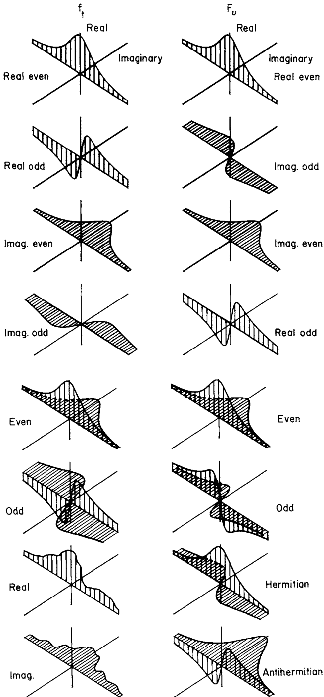
Figure 5.2 Symmetry properties of the DFT using the centered format whereby the indices t and \nu run from -N/2 to N/2 - 1 . For even N , the center of symmetry occurs at t and \nu = 0 .
