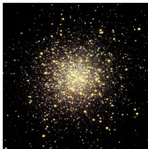
Globular Cluster M13
