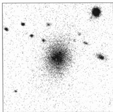
Fig. 1 e: FCC #156
